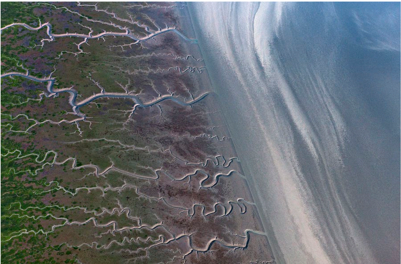
Figure 1. Parallel tidal channel patterns cutting through tidal-flat and salt-marsh surfaces. What controls the size and spacing of channels like these? How will climate change and human interference affect these patterns?
